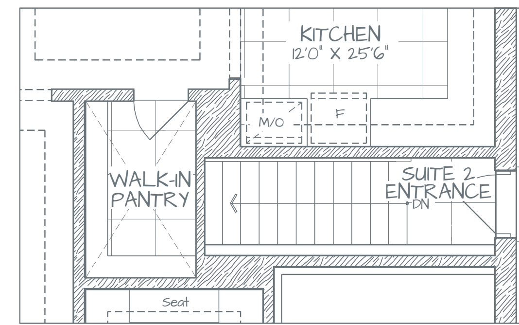
PART. OPT. GROUND FLOOR W/SEPARATE LOWER LEVEL ENTRY
