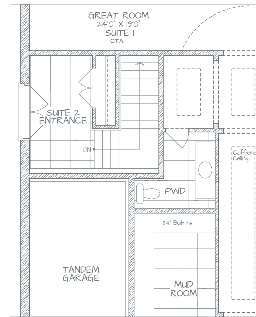
PART. OPT. GROUND FLOOR WITH SECONDARY SUITE
